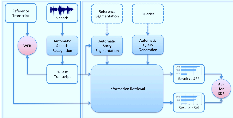
Figure 1.3: Overview of a proposed novel framework for to ASR-for-SDR evaluation without the use of qrels or a need for manually generated queries and story boundaries.
